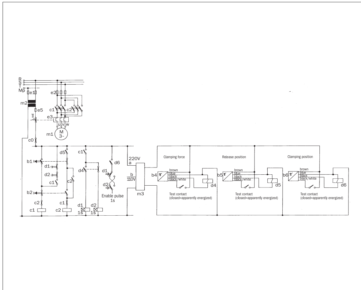
Basic circuit diagram
